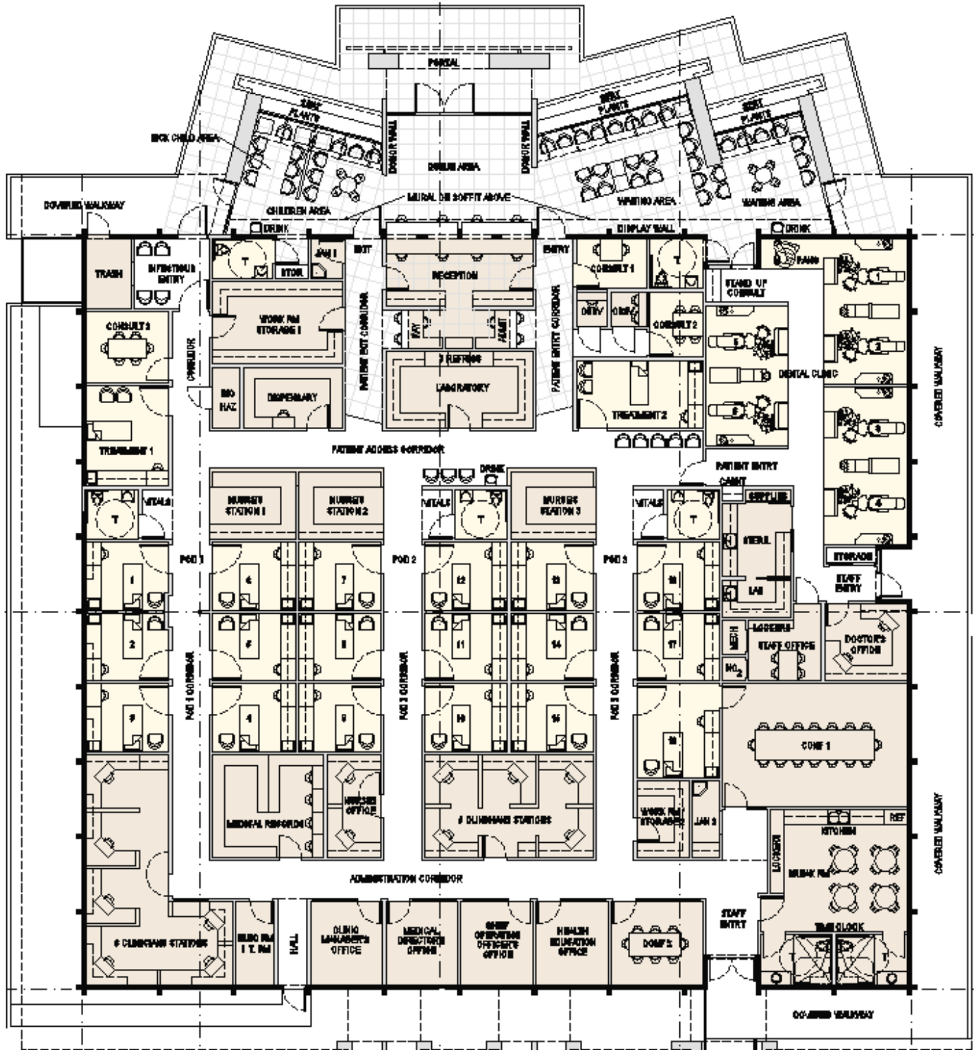
Schematic Floor Plan
